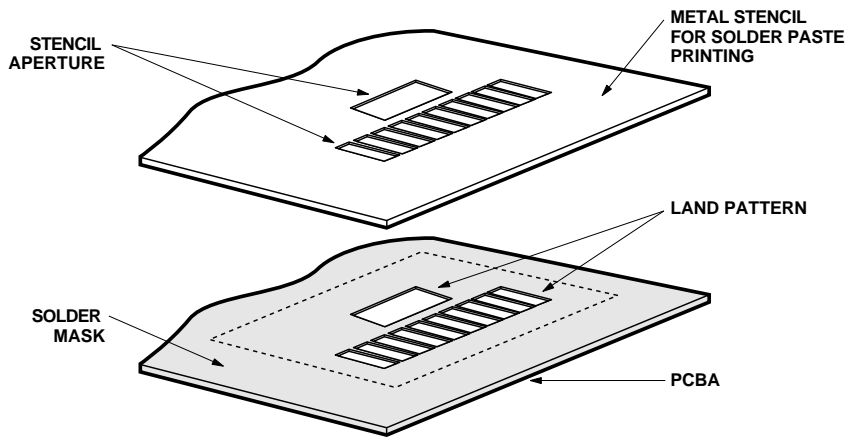
Figure 1.0. Stencil and PCBA.
