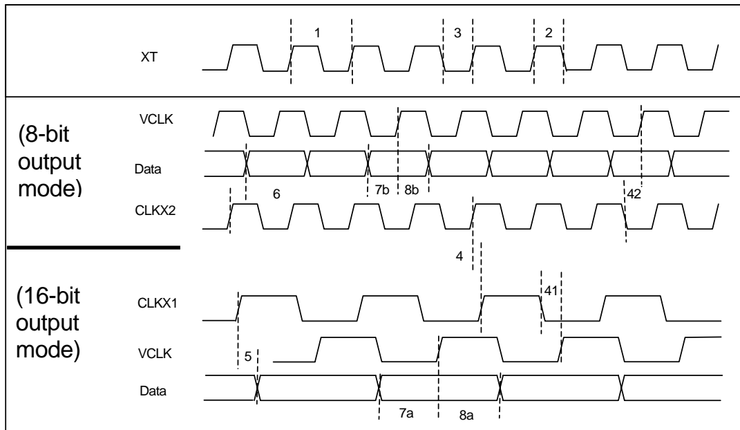
Clock Timing Diagram
