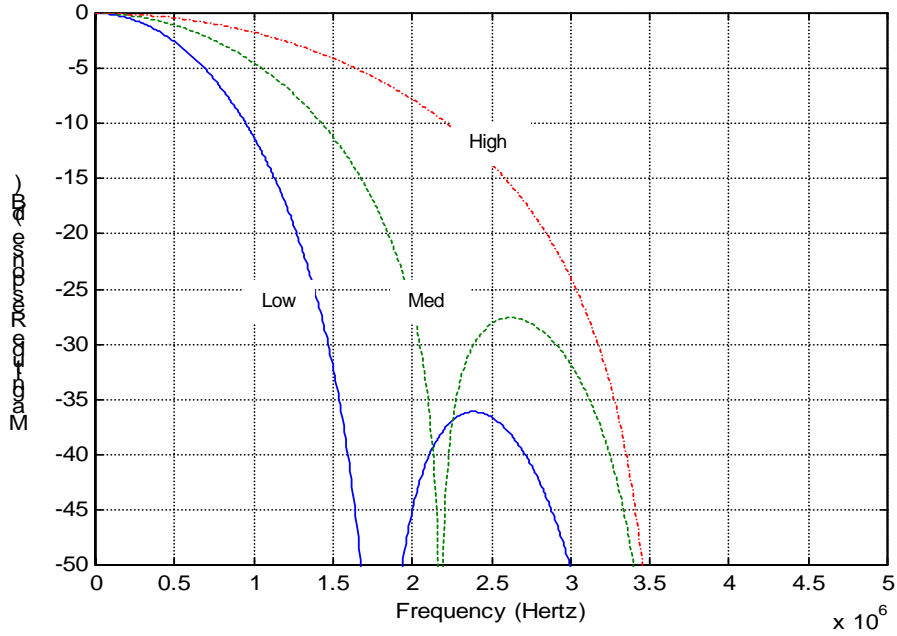
Horizontal Scaler Pre- Filter curves
