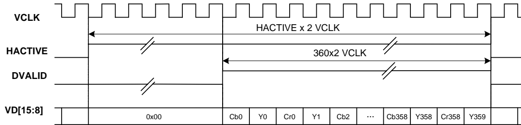
Figure 2. 8 bit mode Horizontal Down Scaling Output
