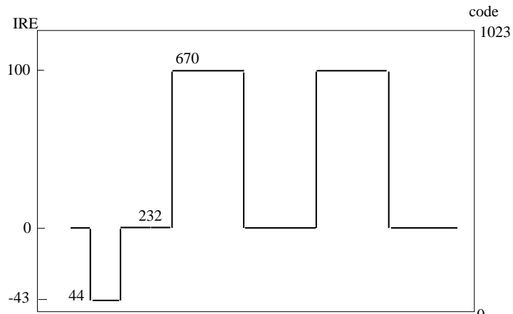
Analog R output level(625/50 system) 100%amplitude,100%saturation color bar
