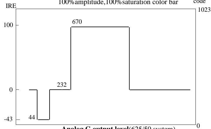
Analog G output level(625/50 system) 100%amplitude,100%saturation color bar
