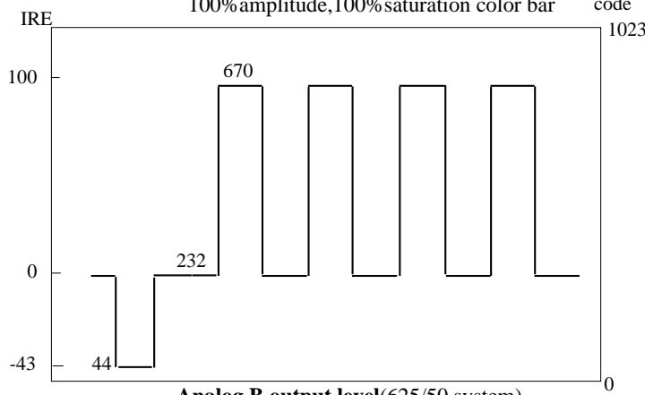
Analog B output level(625/50 system) 100%amplitude,100%saturation color bar
