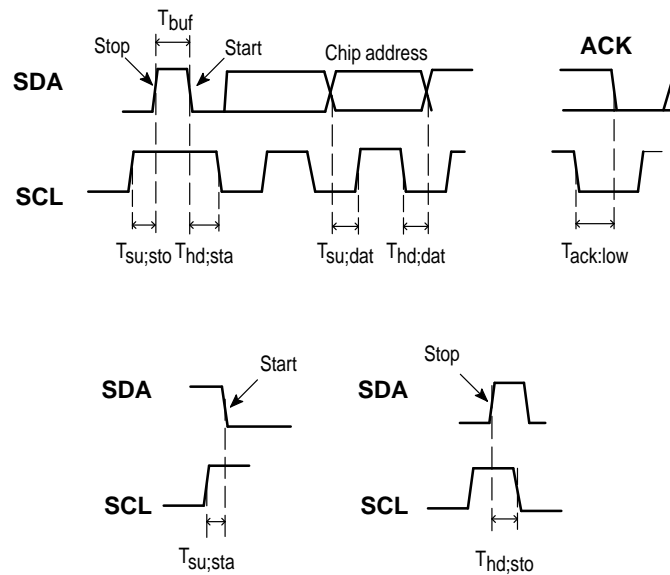
Figure 3. Timings Definition
