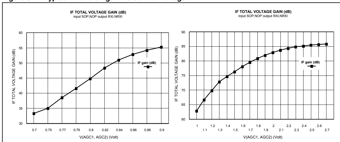
Figure 3. Typical IF overall gain vs control voltage
