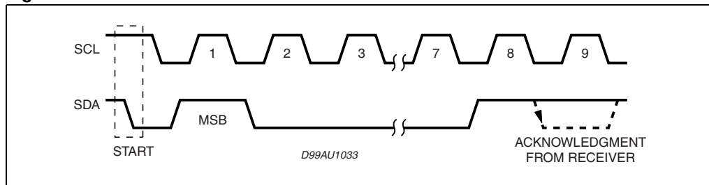
Figure 7. Ack on I 2 Cbus
