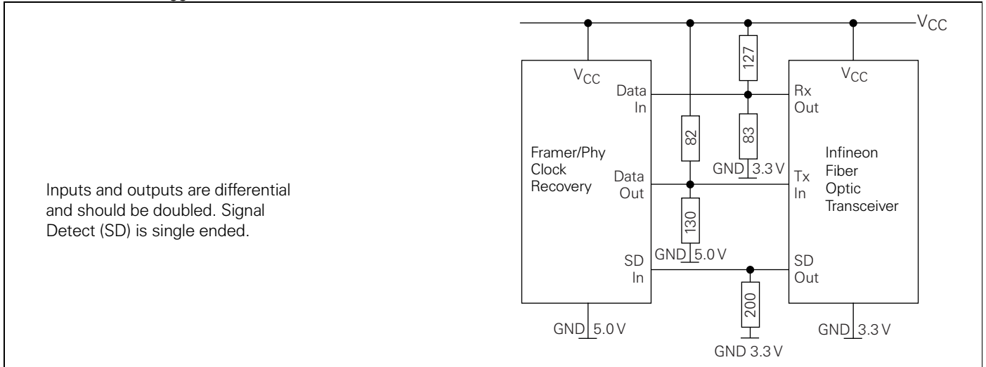
Figure 2. Common VCC
