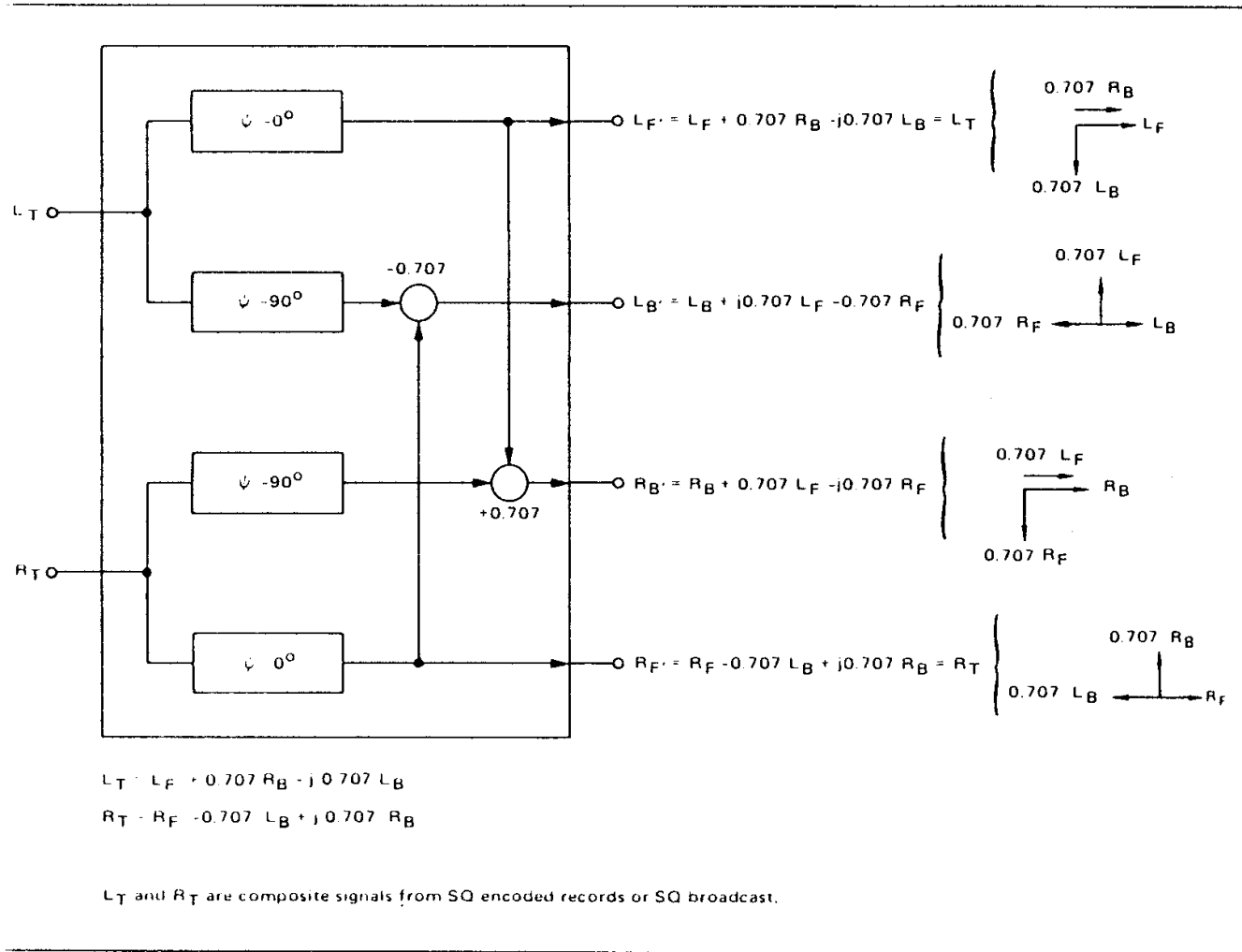
FIGURE 4 – DECODING PROCESS DIAGRAM
