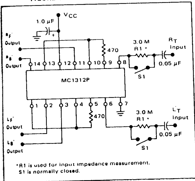
FIGURE 2 - MC1312P TEST CIRCUIT
