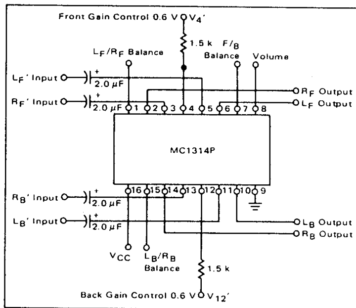
FIGURE 5 – MC1314P TEST CIRCUIT
