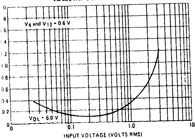
FIGURE 10 - TOTAL HARMONIC DISTORTION versus INPUT VOLTAGE
