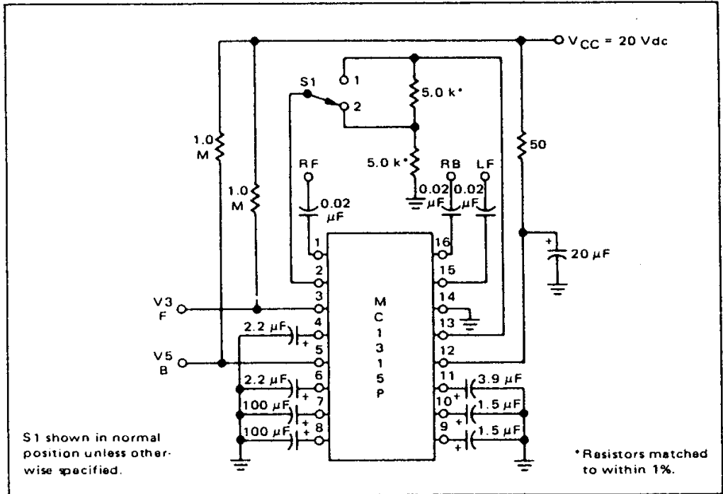
FIGURE 12 – MC1315P TEST CIRCUIT
