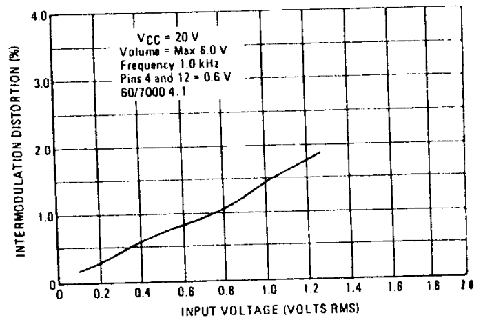
FIGURE 9 - INTERMODULATION DISTORTION versus INPUT VOLTAGE
