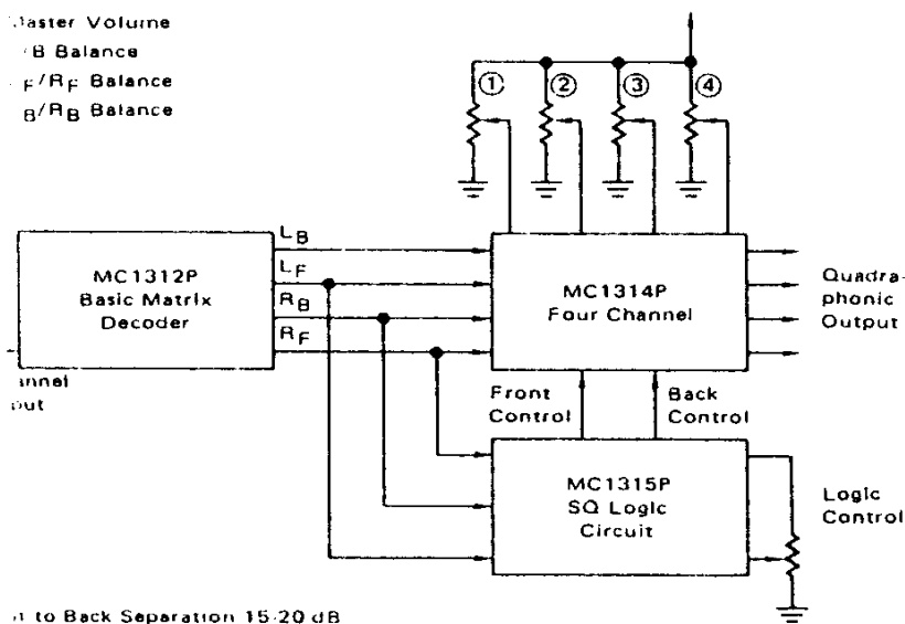
FIGURE 1 - SQ LOGIC DECODER SYSTEM
