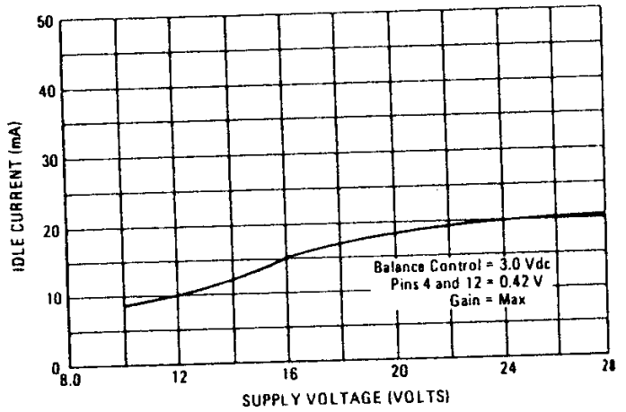
FIGURE 7 - IDLE CURRENT versus SUPPLY VOLTAGE
