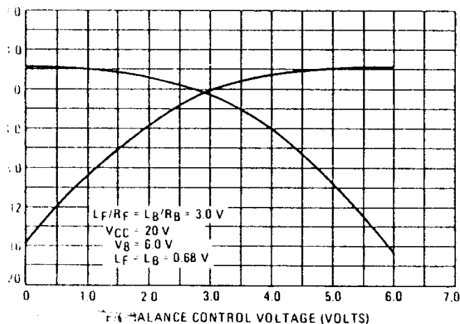
FIGURE 15 – GAIN versus F/B BALANCE
