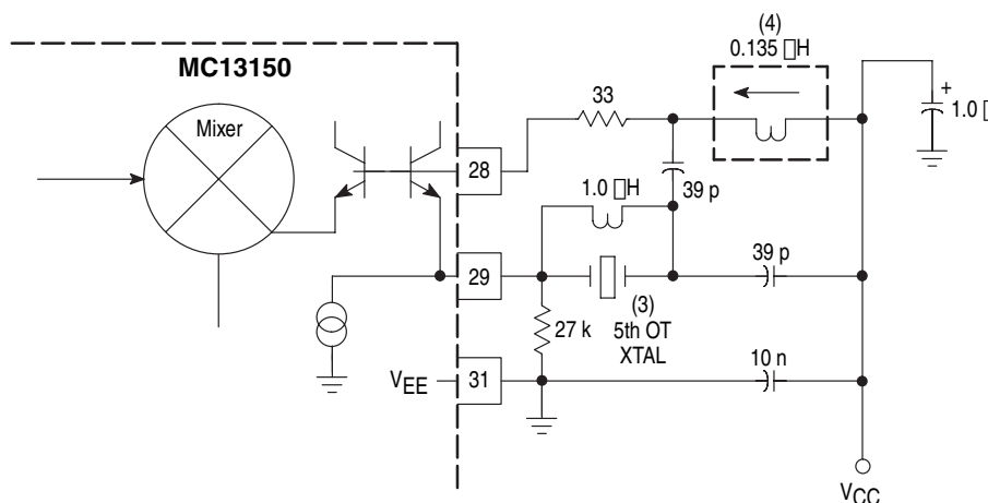
Figure 16. ML13150 Overtone Oscillator f_{RF} = 83.16 \text{ MHz} ; f_{LO} = 83.616 \text{ MHz} 5th Overtone Crystal Oscillator
