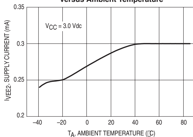
Figure 20. Supply Current, I_{VEE2} versus Ambient Temperature
