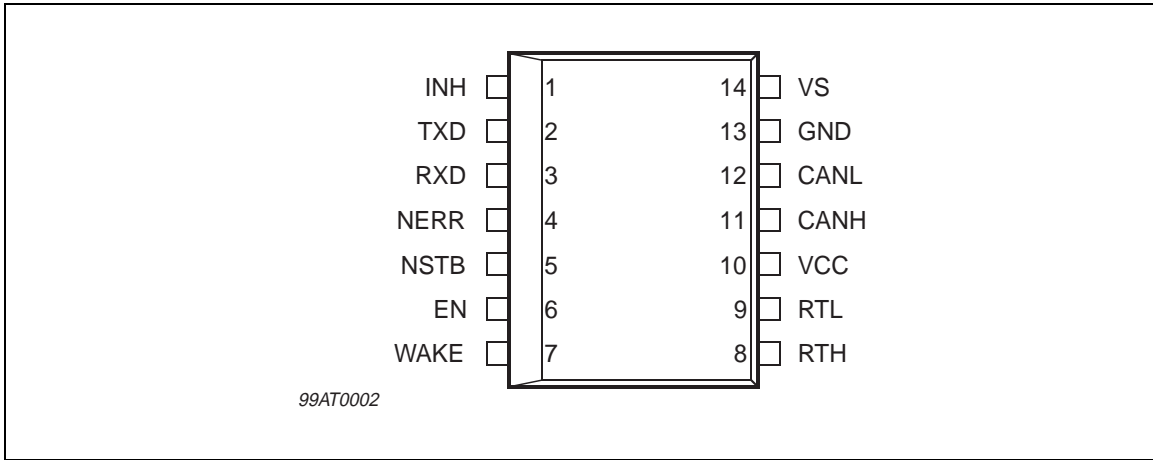
Figure 2. Pin Connection top view.
