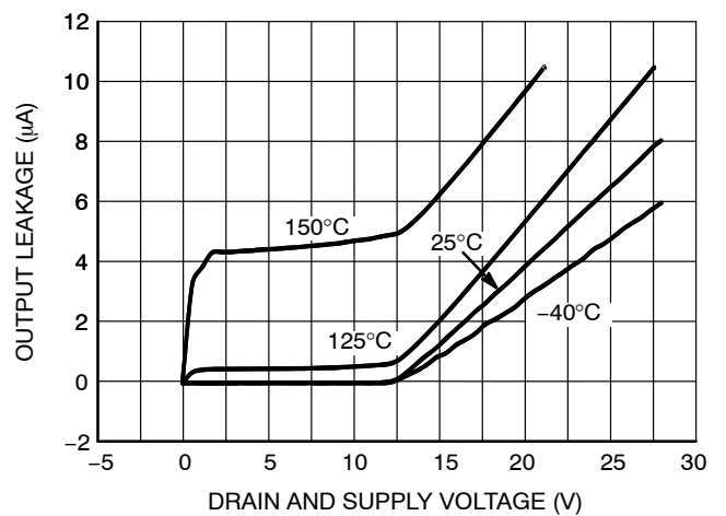
Figure 15. Standby Output Leakage vs. VS
