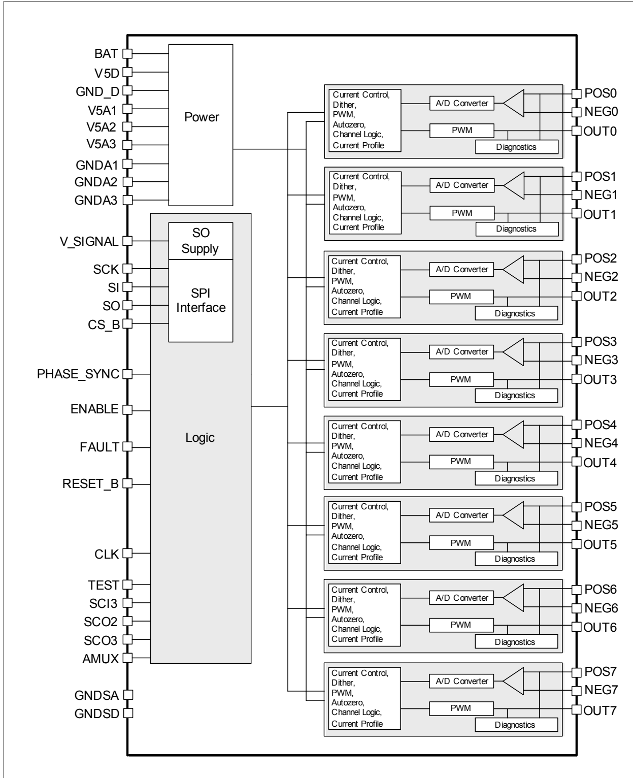
Figure 5 Block Diagram
