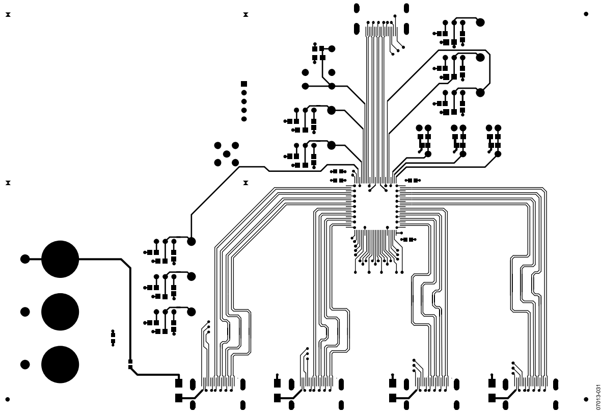
Figure 31. Layout of the TMD5 Traces on the AD8191A Evaluation Board (Only Top Signal Routing Layer is Shown)
