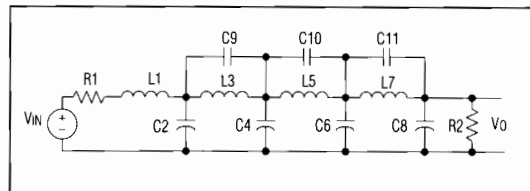
Figure 2. 8th-Order Ladder Filter Network
