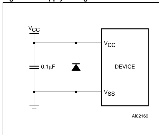
Figure 14. Supply Voltage Protection
