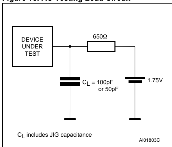
Figure 15. AC Testing Load Circuit
