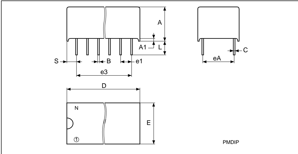
Figure 17. PMDIP32 – 32-pin Plastic DIP Module, Package Outline
