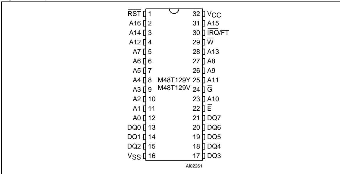
Figure 3. 32-pin Module Connections
