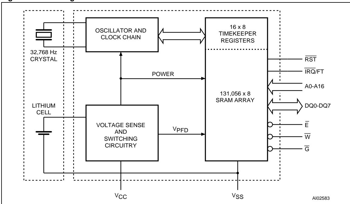
Figure 4. Block Diagram
