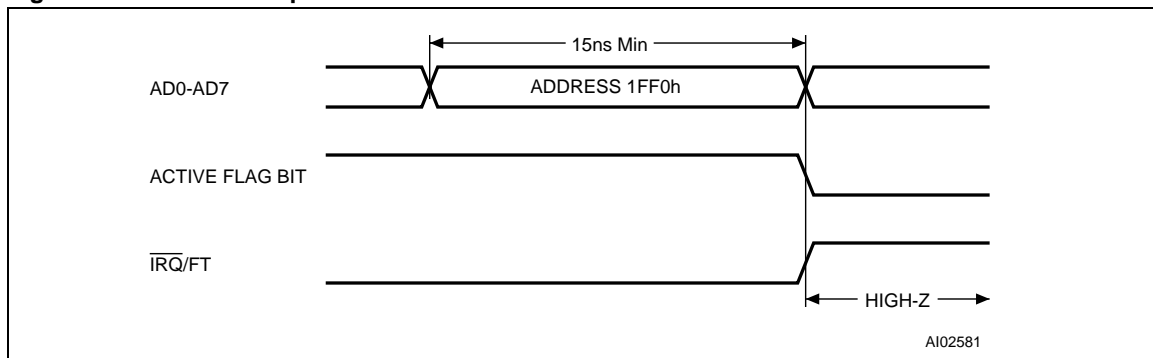
Figure 12. Alarm Interrupt Reset Waveform
