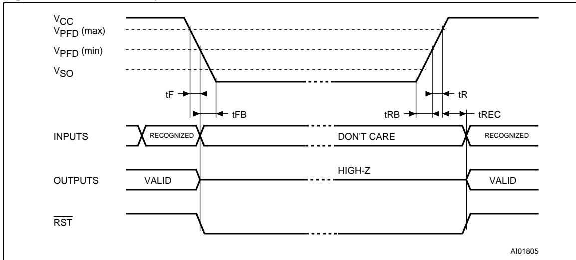
Figure 16. Power Down/Up Mode AC Waveforms
