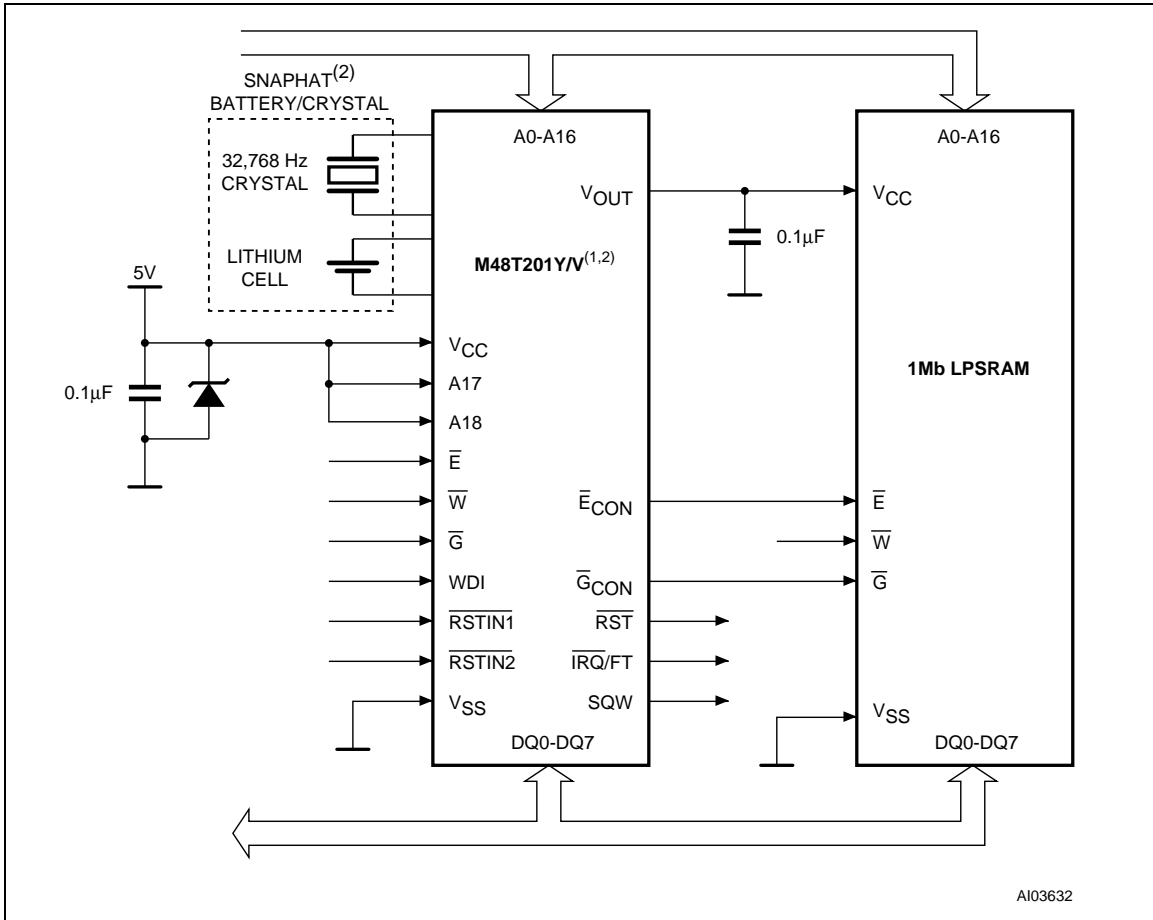
Figure 5. Hardware Hookup for Equivalent Surface-mount (SMT) Solution
