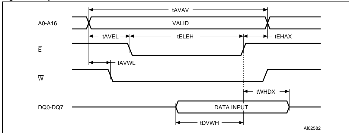
Figure 9. Chip Enable Controlled, WRITE AC Waveforms
