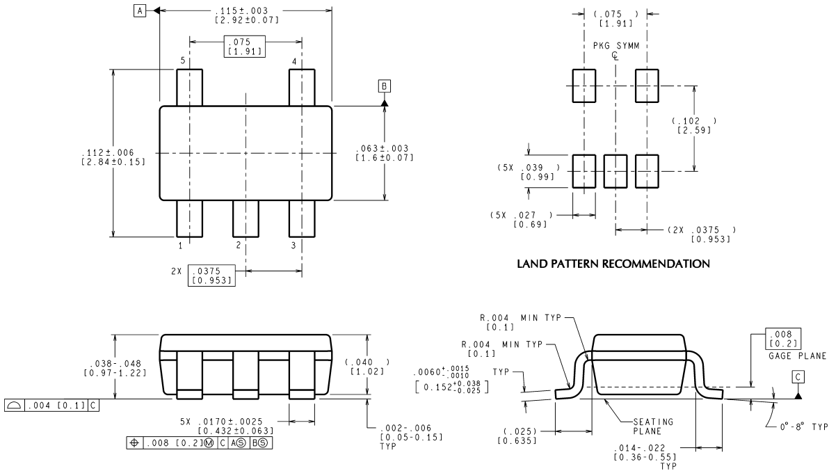
5-Pin SOT23 NS Product Number MF05A
