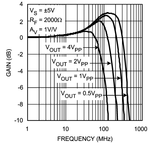
Frequency Response vs. V_{OUT} , A_V = 1
