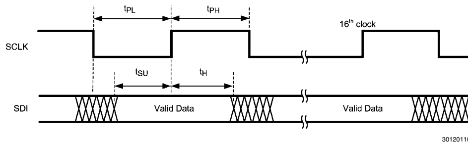
FIGURE 13. Write Timing Data Written to SDI Pin
