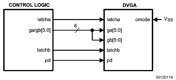
FIGURE 9. Parallel Mode Connection Using Latch Pins to Mux Digital Data
