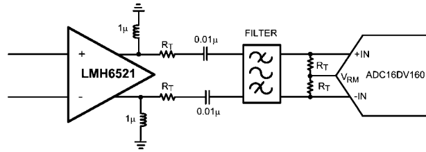
FIGURE 5. Example Output Configuration
