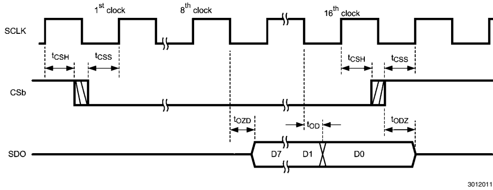
FIGURE 12. Read Timing
