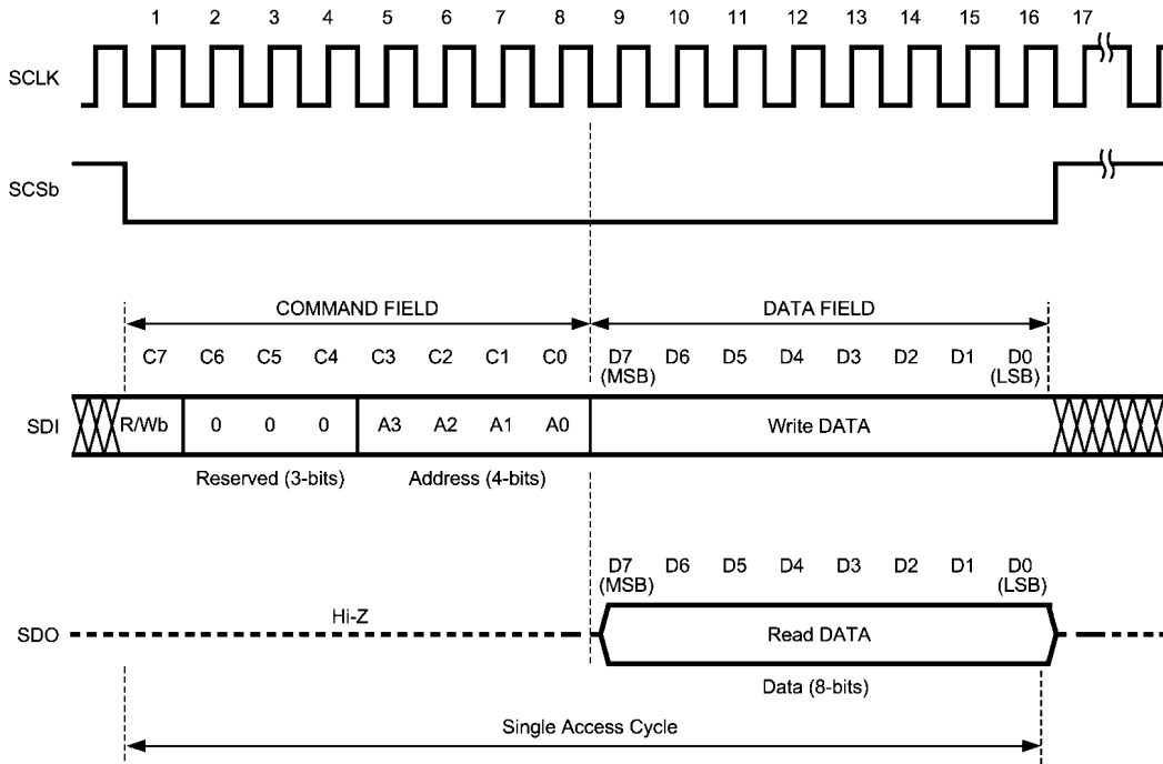
FIGURE 10. Serial Interface Protocol (SPI compatible)
