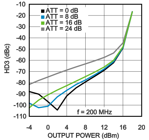
Third Order Harmonic Distortion at 200 MHz
