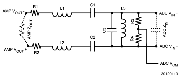
FIGURE 17. Sample Bandpass Filter
