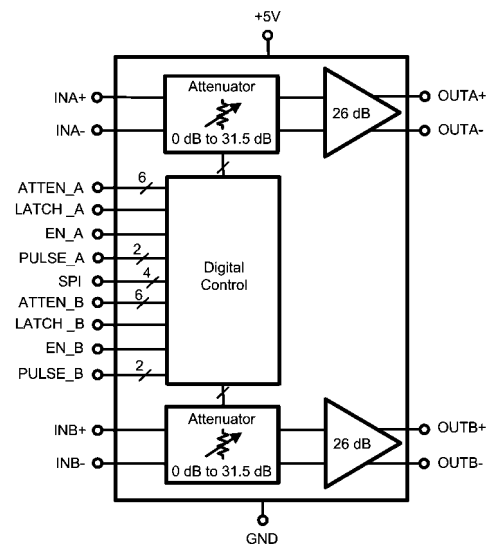
FIGURE 3. LMH6521 Block Diagram
