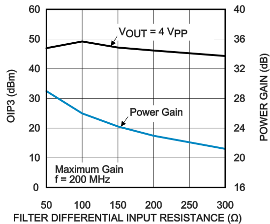
FIGURE 6. OIP3 vs Amplifier Load Resistance
