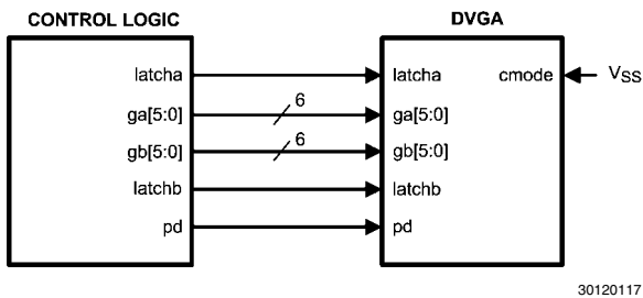
FIGURE 7. Parallel Mode Connection for Fastest Response
