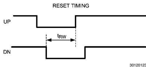
FIGURE 15. Pulse Mode Timing
