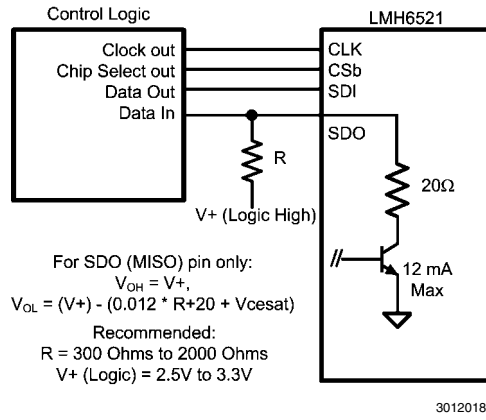
FIGURE 11. Serial Mode 4-wire Connection
