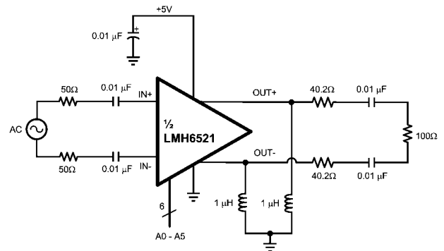
FIGURE 2. Basic Operating Connection
