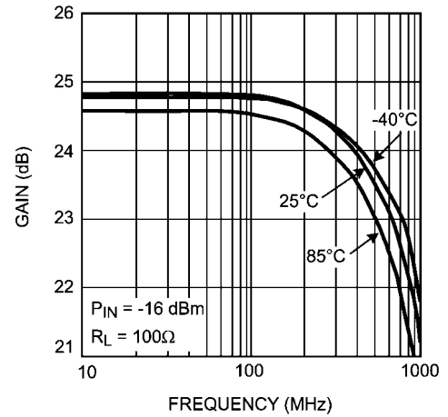
Frequency Response over Temperature, Maximum Gain
