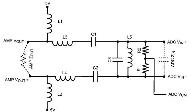
FIGURE 10. Sample Filter
