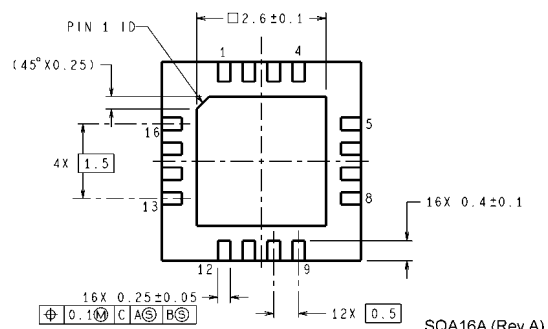
16-Pin Package NS Package Number SQA16A
