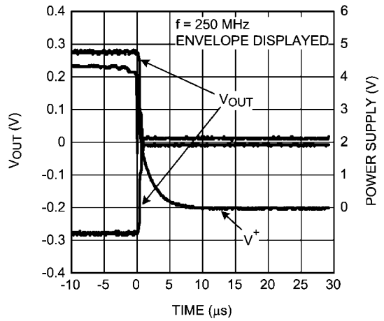
Power Off Timing, Minimum Gain
