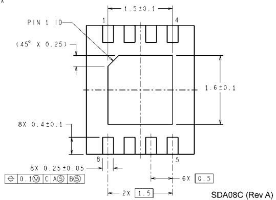
8-Pin LLP NS Package Number SDA08C
