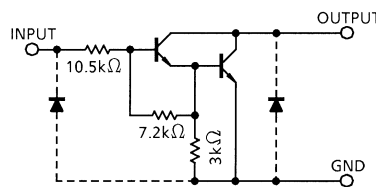
TD62104P / F
