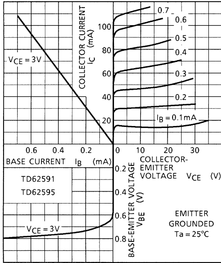
STATIC CHARACTERISTICS
