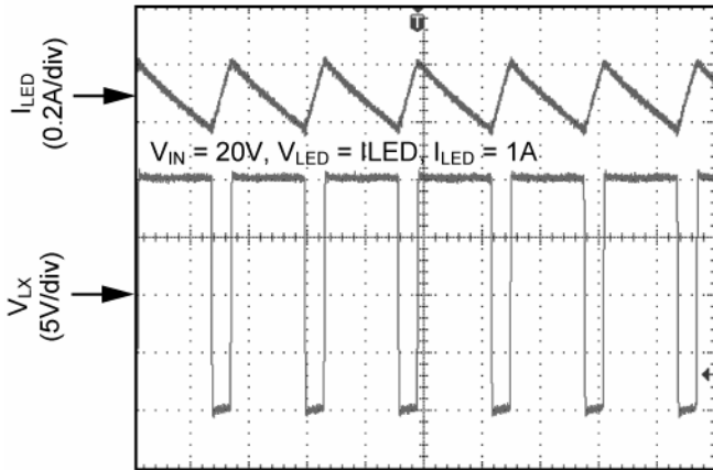
I_{LED} and V_{LX} @ V_{IN} = 20V
