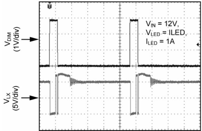
20kHz Dimming @ 10% Duty
