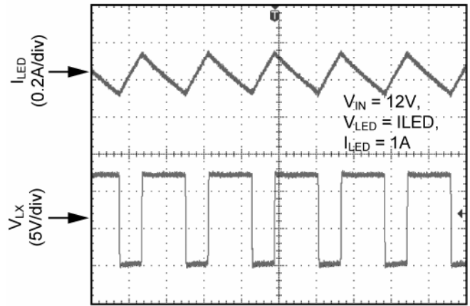
I_{LED} and V_{LX} @ V_{IN} = 12V
