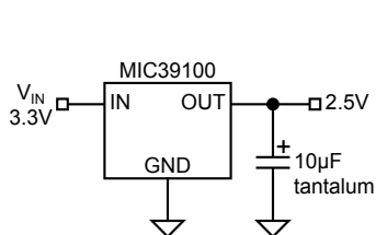
2.5V/1A Regulator
