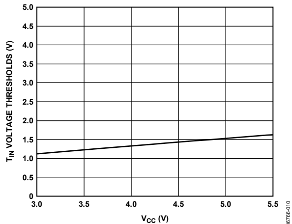
Figure 10. T IN Voltage Threshold vs. V CC
