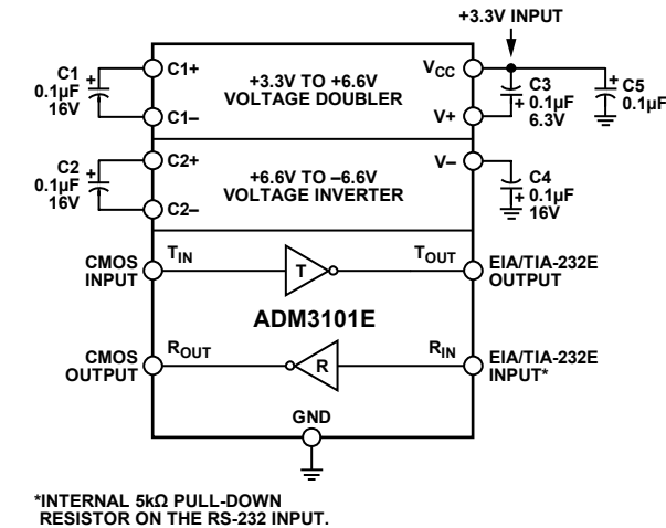
Figure 11. ADM3101E Typical Operating Circuit
