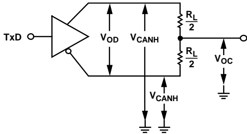
Figure 22. Driver Voltage Measurement
