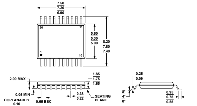
Figure 27. 20-Lead Shrink Small Outline Package [SSOP] (RS-20) Dimensions shown in millimeters
