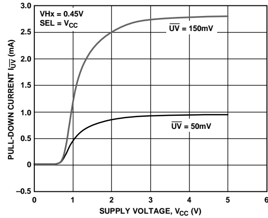
Figure 13. I_{SINK} , I_{UV} vs. V_{CC}
