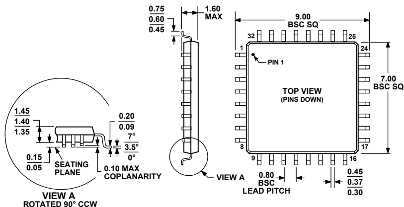
COMPLIANT TO JEDEC STANDARDS MS-026-BBA Figure 47. 32-Lead Low Profile Quad Flat Package [LQFP] (ST-32-2) Dimensions shown in millimeters
