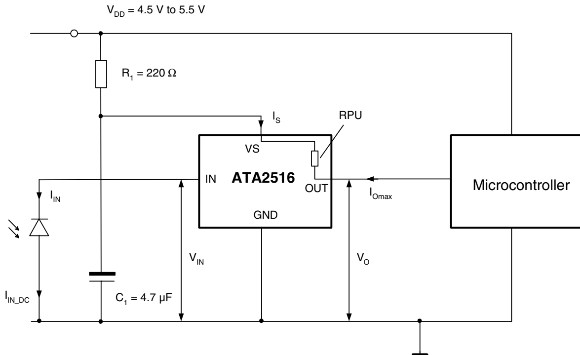
Figure 3. Application Circuit
