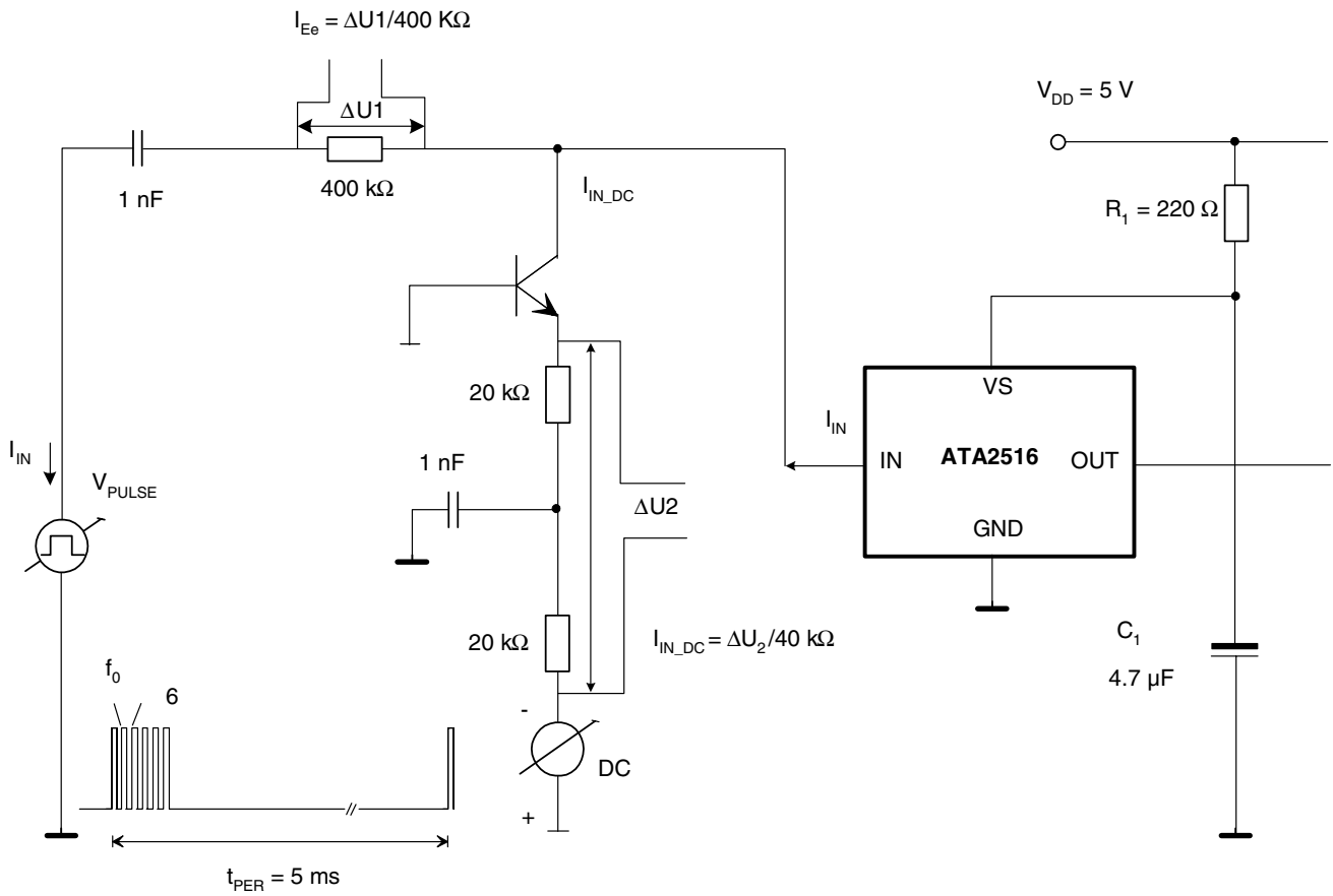
Figure 4. Test Circuit
