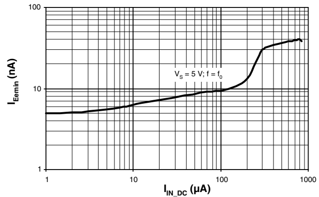
Figure 7. I_{Emin} versus I_{IN\_DC} , V_S = 5\text{ V} , T_{amb} = 25^\circ\text{C}
