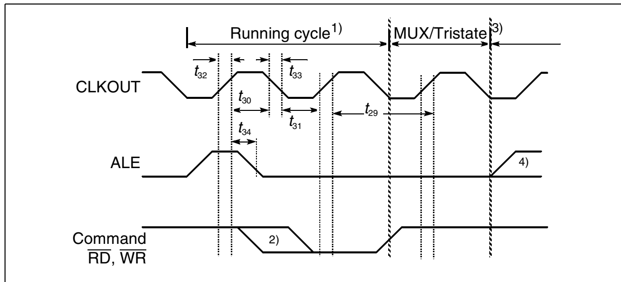
Figure 20 CLKOUT Timing
