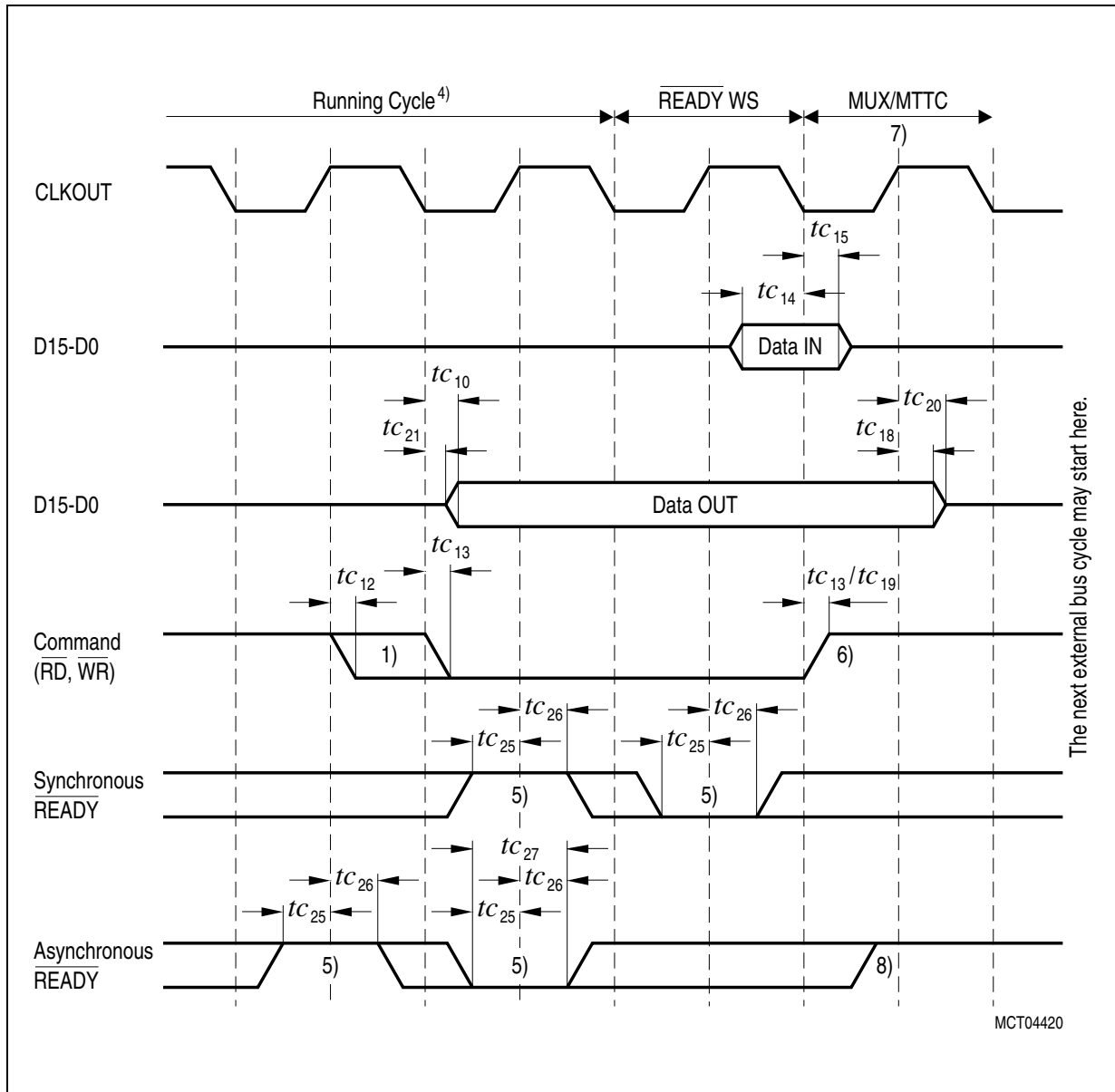
Figure 20 \overline{\text{READY}} Timings
