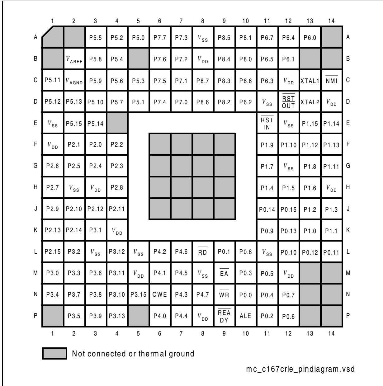
Figure 3 Pin Configuration P-BGA-176-2 (top view)
