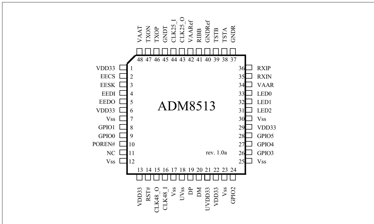
Figure 1 Pin Diagram
