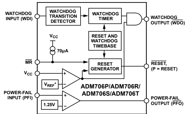
Figure 1. ADM706P/ADM706R/ADM706S/ADM706T
