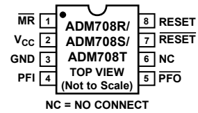
Figure 5. ADM708R/ADM708S/ADM708T
