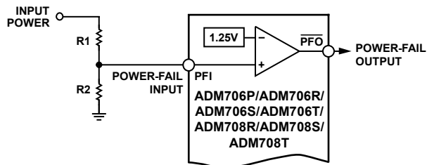
Figure 17. Power-Fail Comparator
