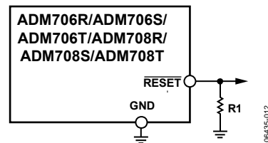
Figure 19. \overline{RESET} Valid Below 1 V
