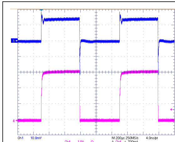
VIN=1.2V, VCNTL=3.3V, VOUT=0.6V @ 3A Sinking
