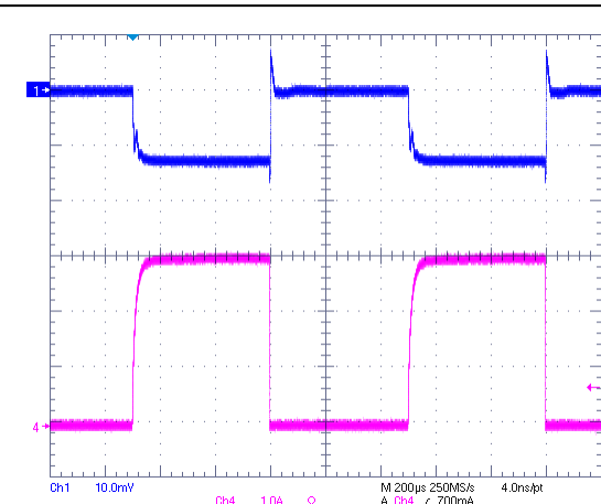
VIN=1.8V, VCNTL=5V, VOUT=0.9V @ 3A Sourcing
