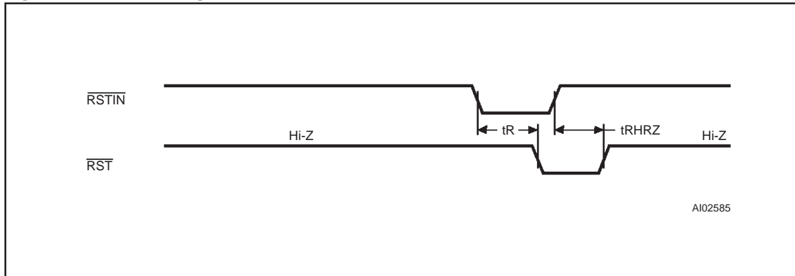
Figure 14. \overline{\text{RSTIN}} Timing Waveform
