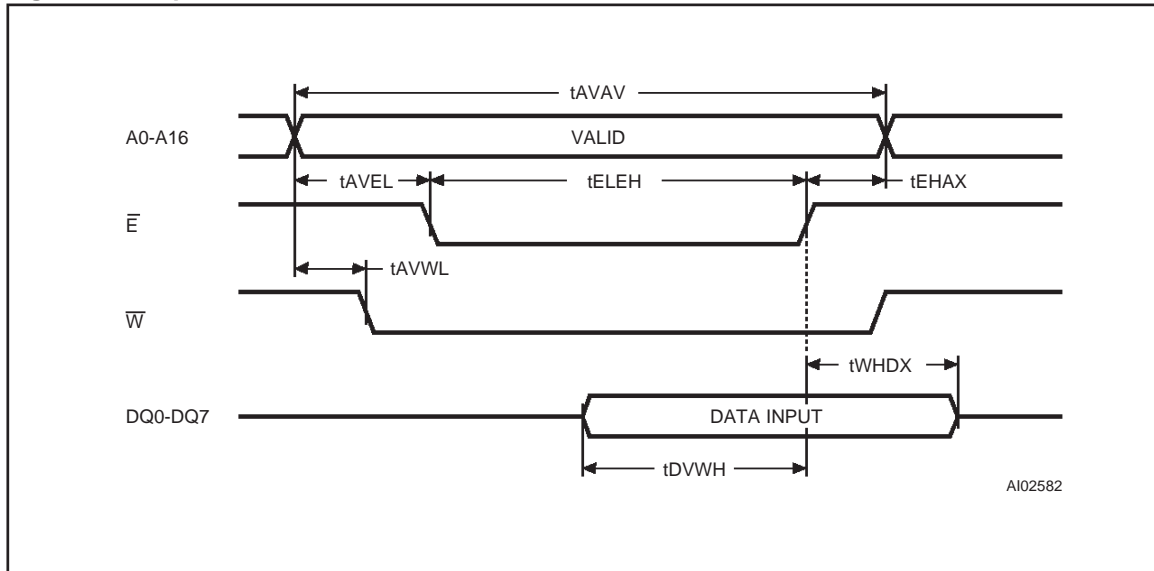
Figure 10. Chip Enable Controlled, Write AC Waveforms
