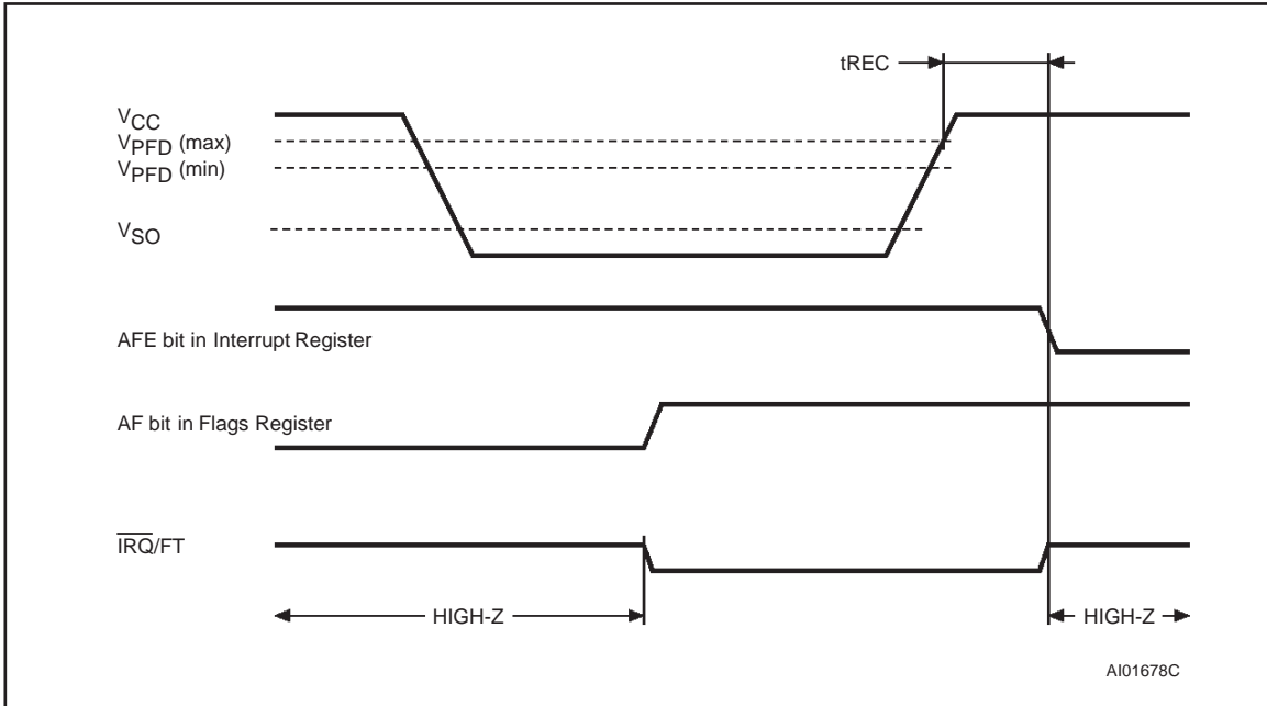
Figure 13. Back-up Mode Alarm Waveforms
