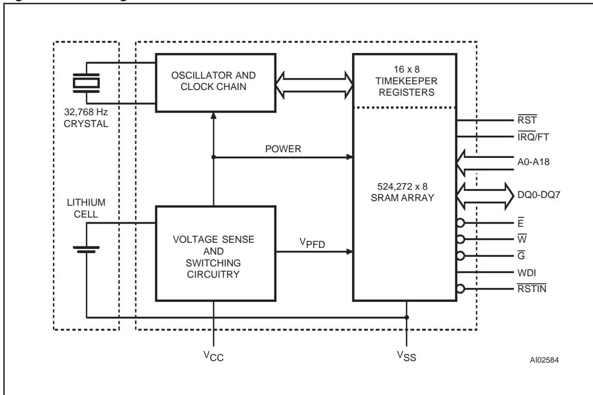
Figure 3. Block Diagram
