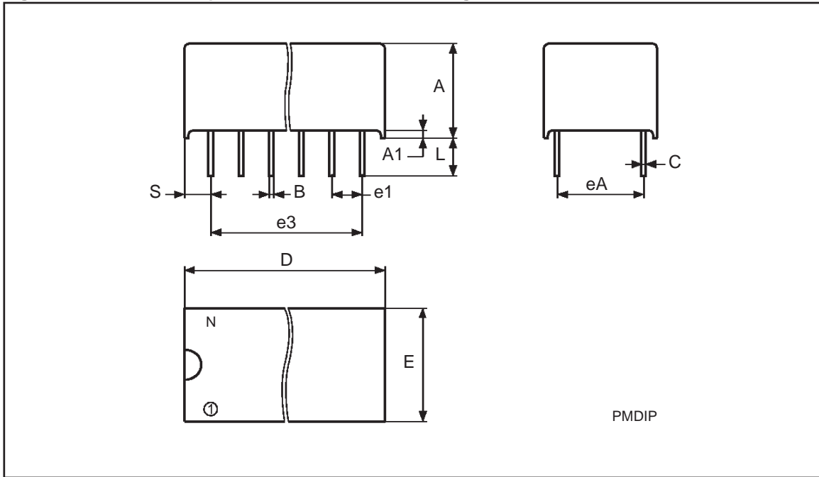
Figure 16. PMDIP32 - 32 pin Plastic Module DIP, Package Outline
