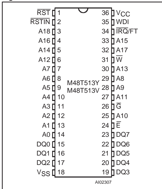
Figure 2. DIP Connections
