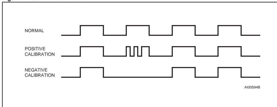
Figure 11. Calibration Waveform
