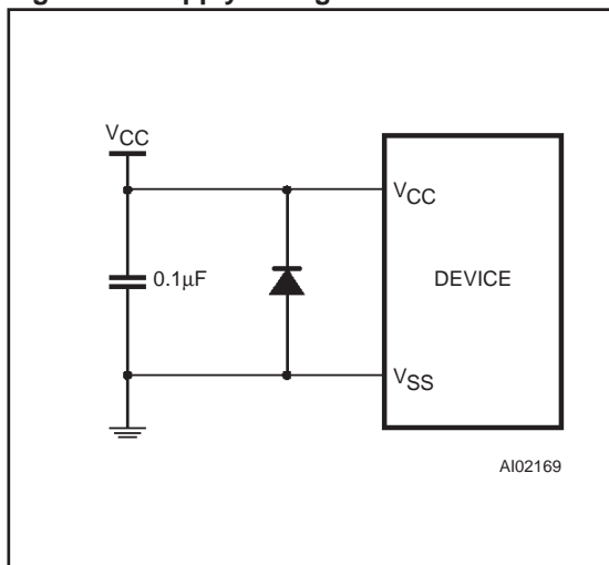
Figure 15. Supply Voltage Protection
