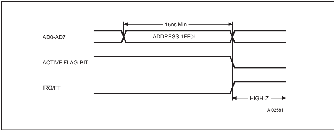
Figure 12. Alarm Interrupt Reset Waveform
