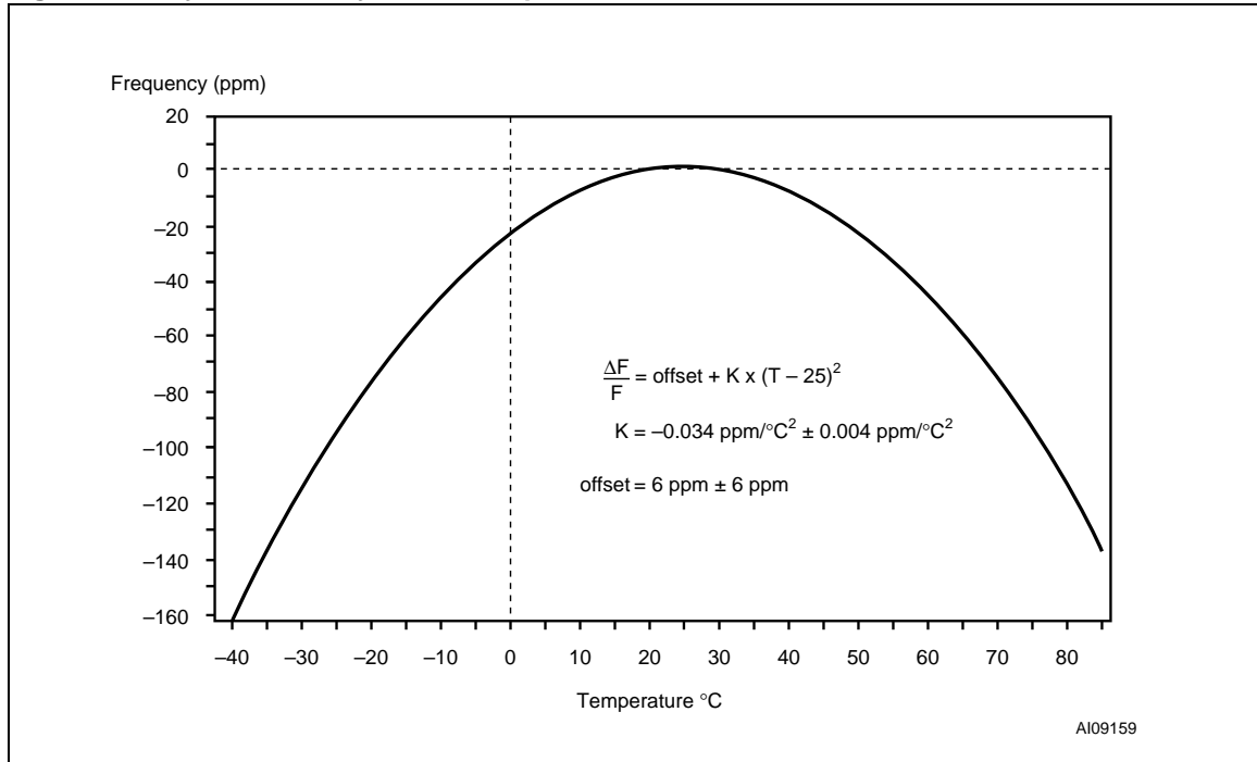
Figure 4. Crystal accuracy across temperature
