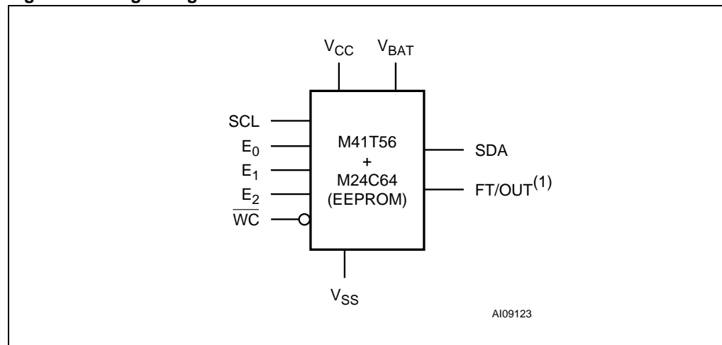
Figure 1. Logic diagram
