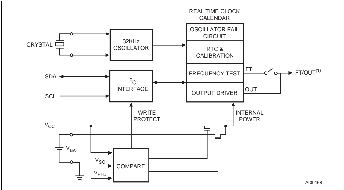
Figure 4. Block Diagram
