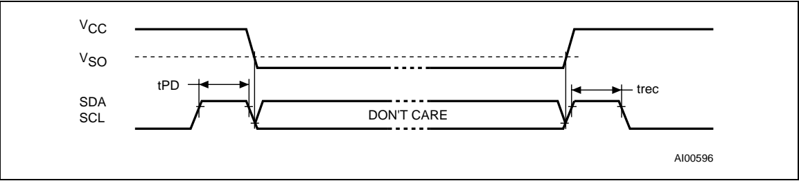
Figure 14. Power Down/Up Mode AC Waveforms
