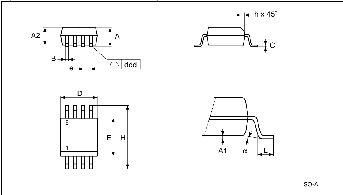
Figure 16. SO8 – 8-lead Plastic Small Package Outline
