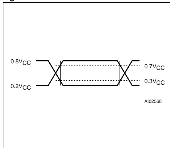
Figure 13. AC Measurement I/O Waveform
