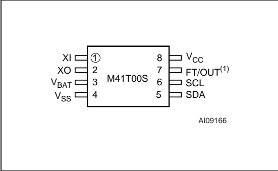
Figure 3. 8-pin SOIC (M) Connections
