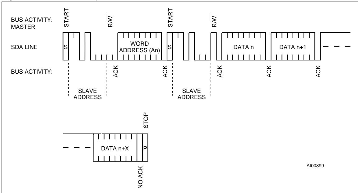
Figure 8. READ Mode Sequence
