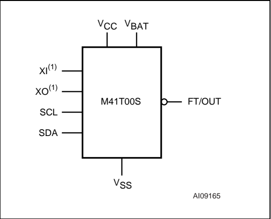
Figure 2. Logic Diagram
