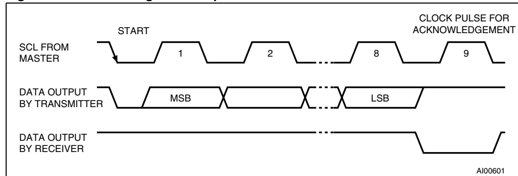
Figure 5. Acknowledgement sequence
