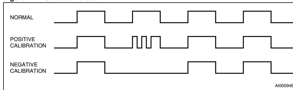
Figure 11. Clock calibration
