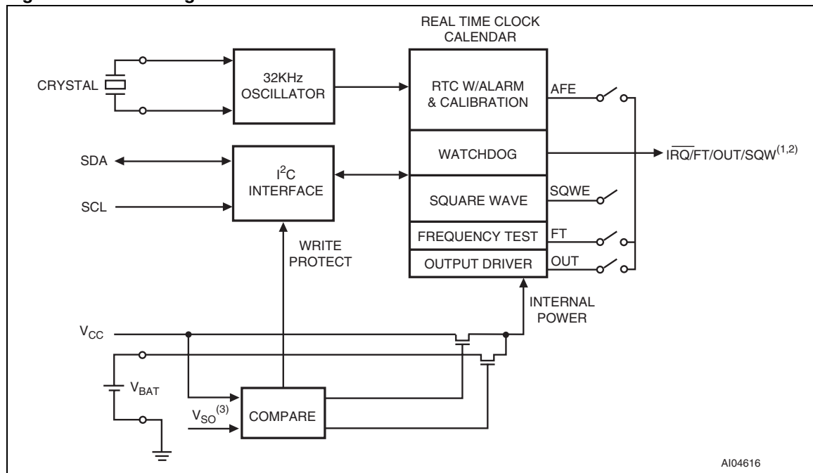
Figure 3. Block diagram
