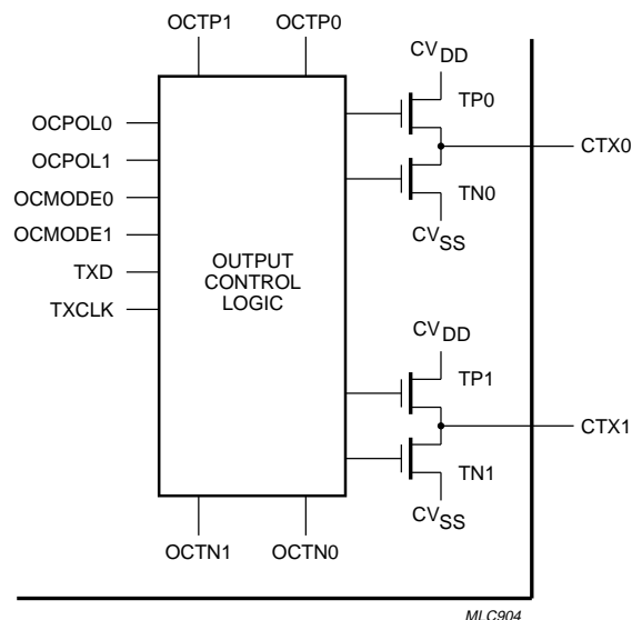
Fig.17 Configurable CAN Transmitter.
