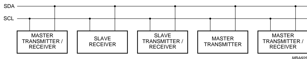
Fig 8. System configuration.
