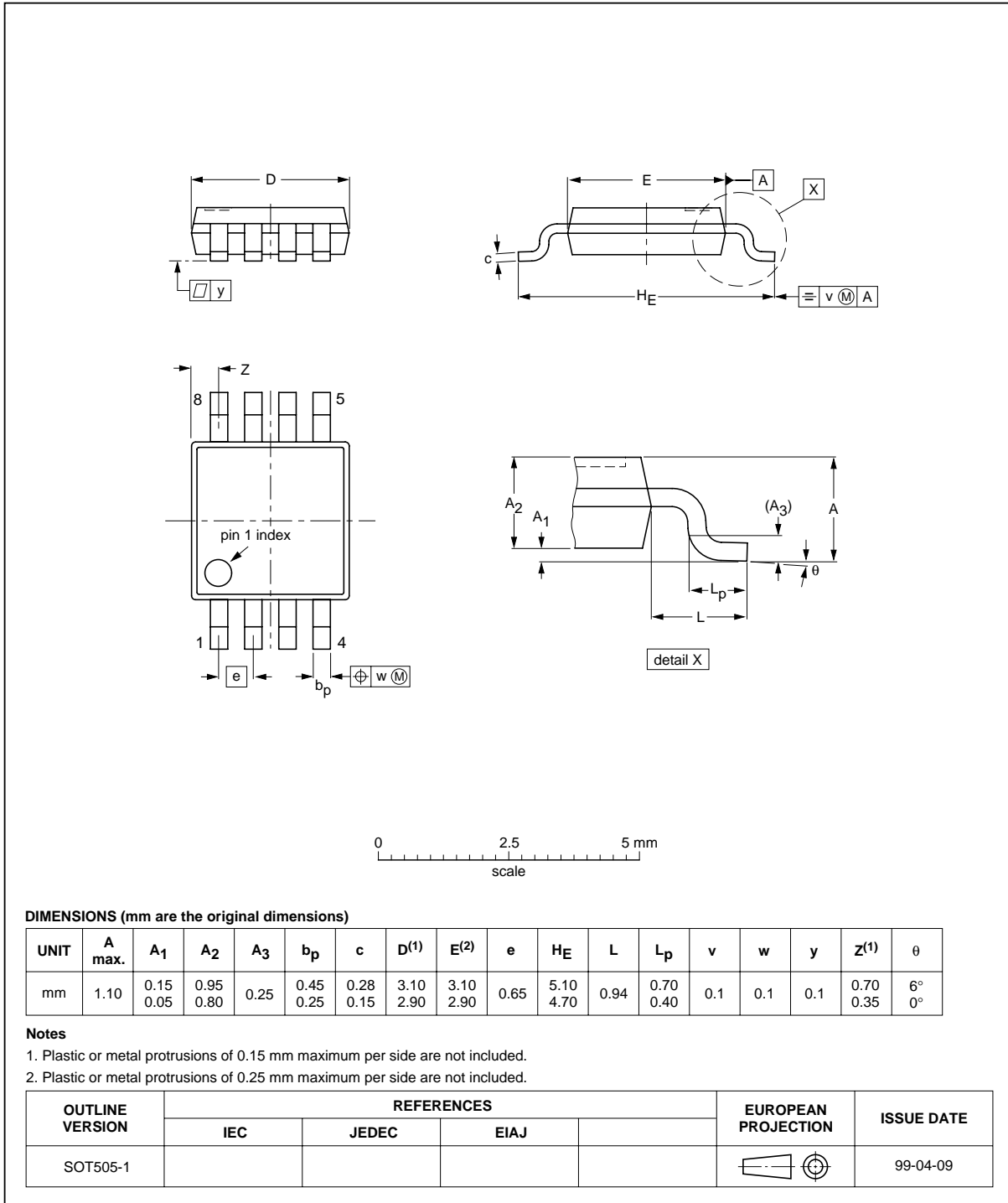
Fig 20. Package outline.
