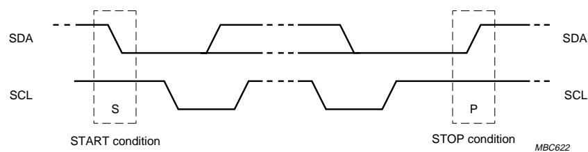
Fig 7. Definition of start and stop conditions.
