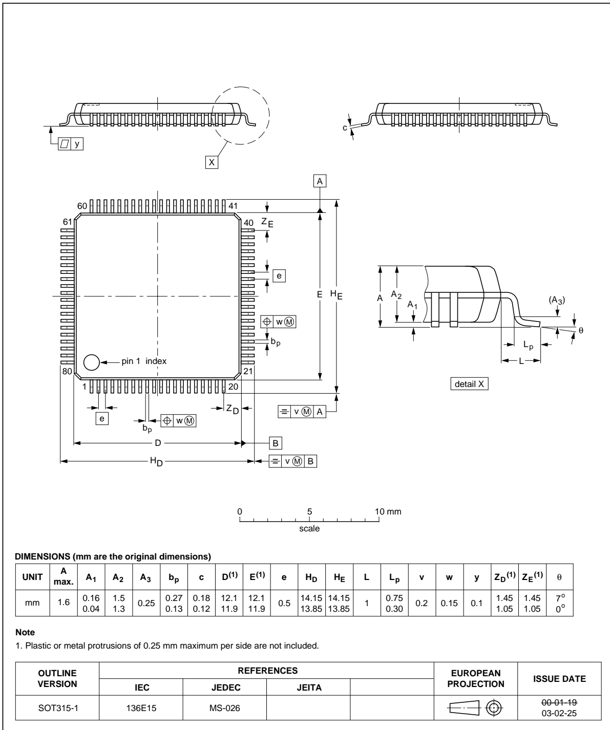
Fig 24. Package outline SOT315-1 (LQFP80)
