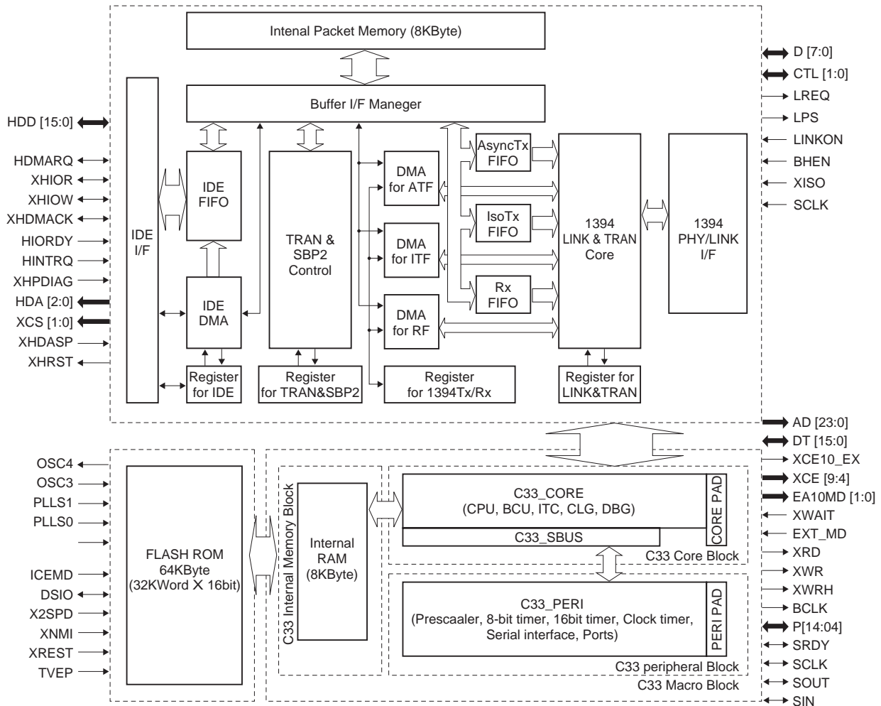
Fig. 3.1 Block diagram
