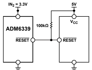
Figure 16. Interfacing with a Different Logic Supply Voltage
