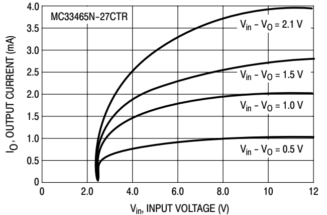
Figure 6. \overline{\text{Reset}} Output Source Current versus Input Voltage
