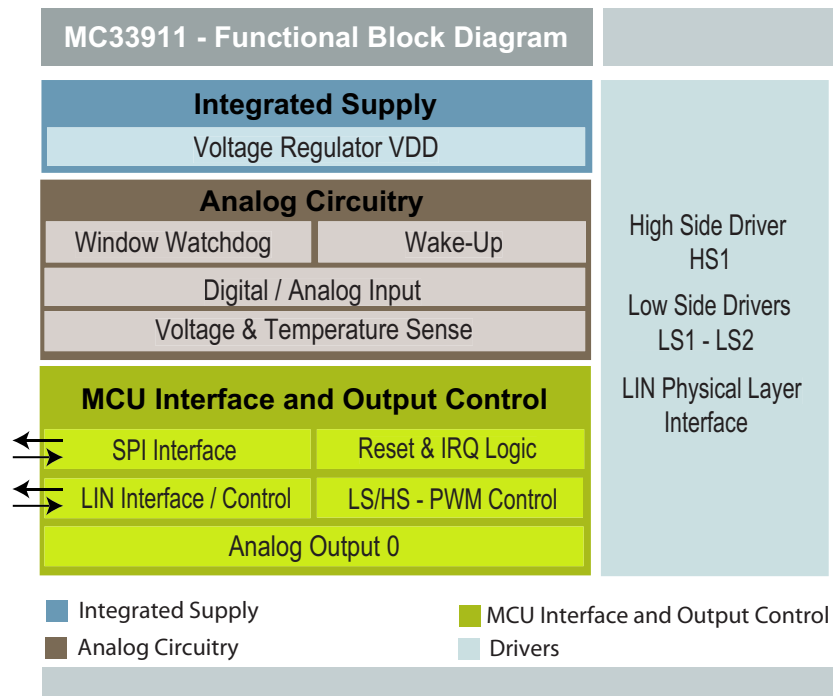
Figure 14. Functional Internal Block Diagram
