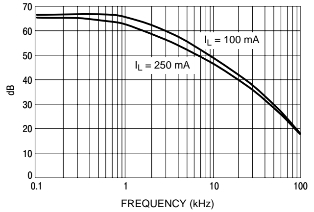
Figure 14. Ripple Rejection
