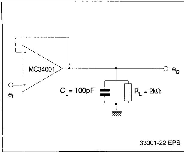
Figure 1 : Voltage Follower
