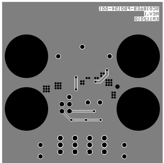
Figure 4 — Bottom Layer Detail
