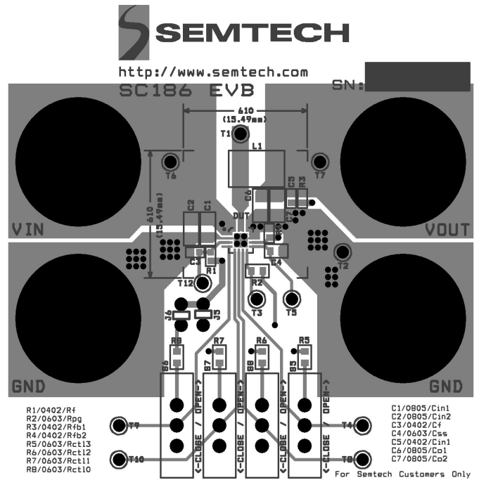
Figure 3 — Recommended PCB Layout (Top Layer)
