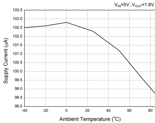
Fig. 3 Supply Current vs. Temperature
