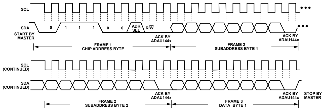
Figure 13. I 2 C Write Clcking
