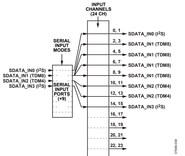
Figure 37. Automatic Input Channel Assignment Example
