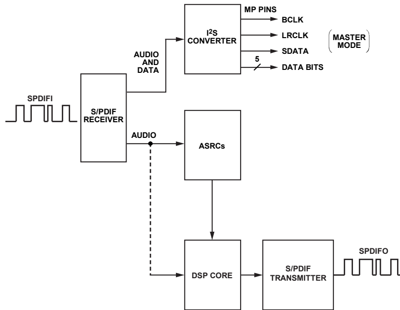
Figure 53. S/PDIF Receiver and Transmitter
