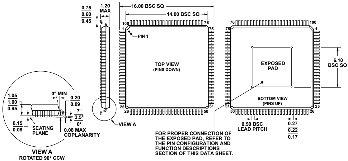
Figure 67. 100-Lead Thin Quad Flat Package, Exposed Pad [TQFP_EP] (SV-100-8) Used for ADAU1442 and ADAU1445 Dimensions shown in millimeters
