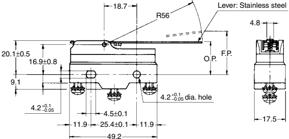
AM1531K (Solder terminal) AM1731K (Screw terminal)
